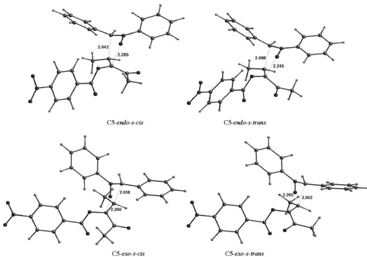
Figure 8. Calculated [B3LYP/6-31G(d)] geometries of the endo and exo C5 TSs for the cycloaddition of the s-cis and s-trans conformations of captodative olefin 12a and nitron 7a .
