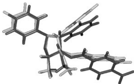
Figure 9. Superposition of the X-ray (dark) and calculated [B3LYP/6-31G(d)] (light) structures of 17a , obtained by superimposing the N-2, C-4, and C-5 atoms of the heterocycle.
