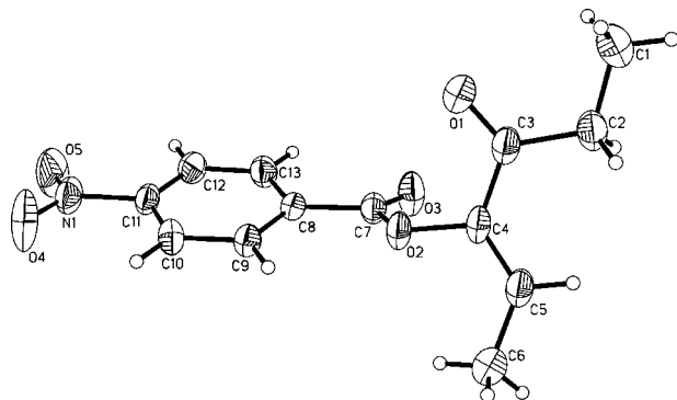
Figure 2. X-ray structure of 12d (ellipsoids with 30% probability).
