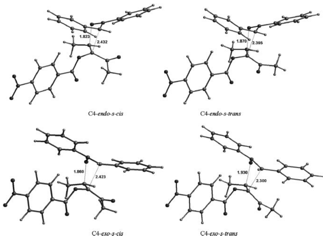
Figure 7. Calculated [B3LYP/6-31G(d)] geometries of the endo and exo C4 TSs for the cycloaddition of the s-cis and s-trans conformations of captodative olefin 12a and nitron 7a .
