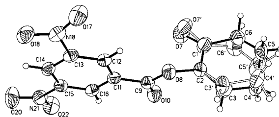
Figure 4. X-ray structure of cyclohexenone 12f (ellipsoids with 30% probability).
