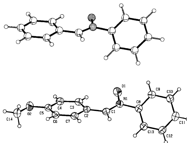
Figure 6. Optimized geometry [B3LYP/6-31G(d)] of nitrone 7a (left) and X-ray structure (right) of 7b (ellipsoids with 30% probability).
