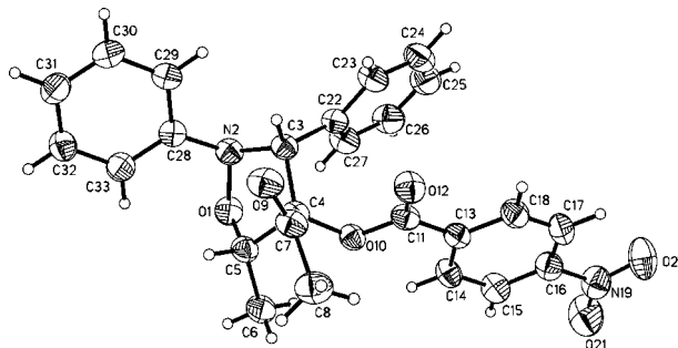
Figure 3. X-ray structure of isoxazolidine 17a (ellipsoids with 30% probability).
