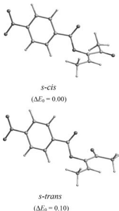
Figure 5. Optimized geometries [B3LYP/6-31G(d)] of olefin 12a for the s-cis and s-trans conformations. In parenthesis the relative zero-point energies ( \text{kcal mol}^{-1} ).
